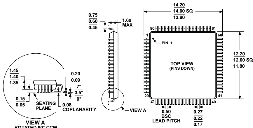
Figure 8. 80-Lead Low Profile Quad Flat Package [LQFP] (ST-80-1) Dimensions shown in millimeters
