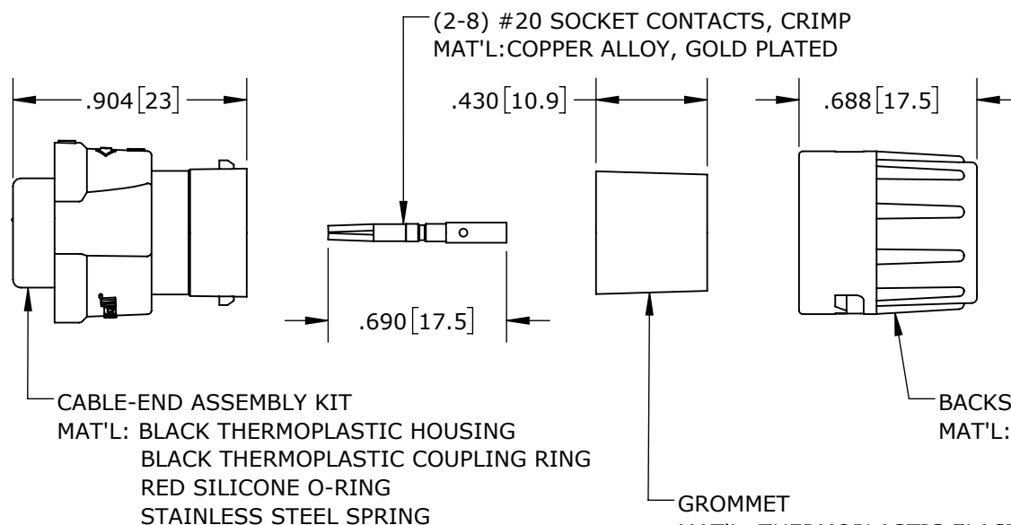
SHOWN ASSEMBLED KIT ASSY: W6280-2SG-P-3XX SHOWN
