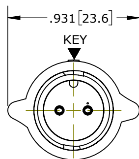
MATING FACE ASSY: W6280-2SG-P-3XX SHOWN
