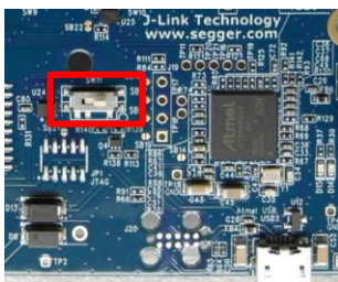
Figure 9: SW11 on development board (showing default position)
