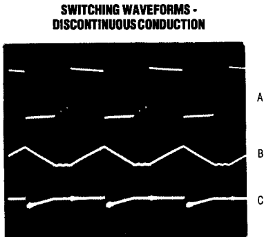
A = Switch Voltage ( L_X ) 5V/div (4.8V to -5.3V) B = Inductor Current, 500mA/div C = Output Voltage Ripple, 50mV/div TIME = 2 \mu\text{s} /div CIRCUIT OF FIG. 1 V_{\text{IN}} = +5\text{V} T_A = +25^\circ\text{C}
