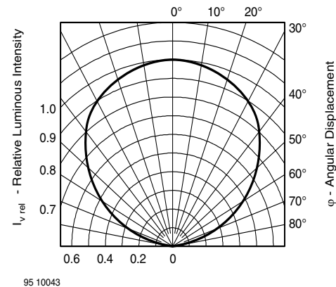
Fig. 2 - Rel. Luminous Intensity vs. Angular Displacement
