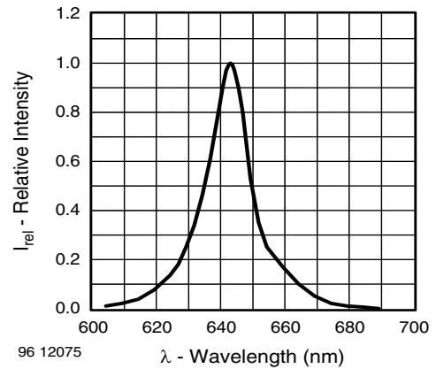
Fig. 6 - Relative Intensity vs. Wavelength
