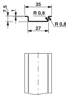
Dimensional drawing
