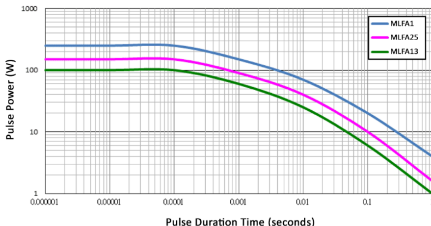
MLFA Series Continuous Pulse ( R \geq 10 ohm)
