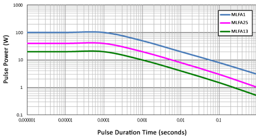
MLFA Series Continuous Pulse (R < 10 ohm)
