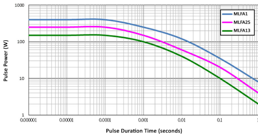
MLFA Series Single Pulse (R ≥ 10 ohm)
