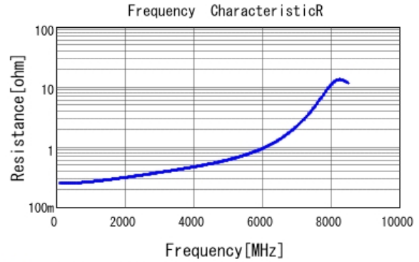
■ GCM1555C1H4R3BA16 R DCOV, 25degC
