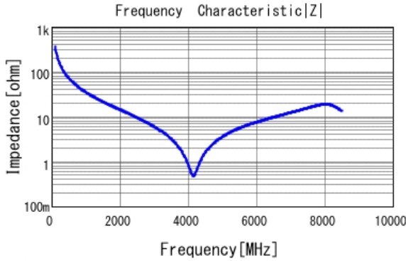
■ GCM1555C1H4R3BA16 |Z| DCOV, 25degC
