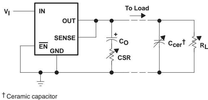
† Ceramic capacitor Figure 6. Test Circuit for Typical Regions of Stability (Refer to Figures 29 through 32)
