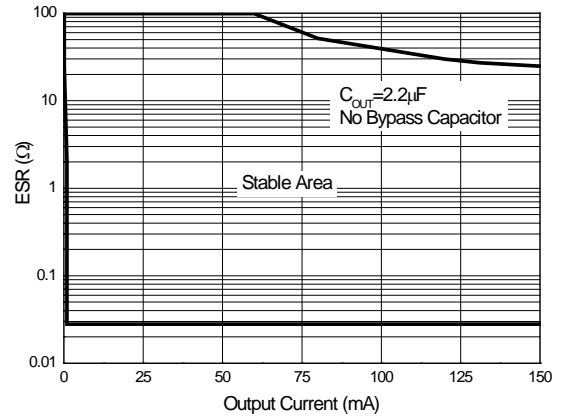
ESR vs. Output Current
