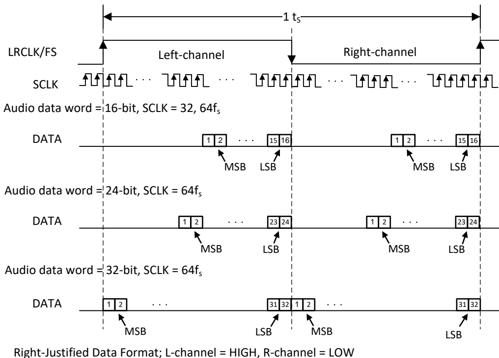
Right-Justified Data Format; L-channel = HIGH, R-channel = LOW
