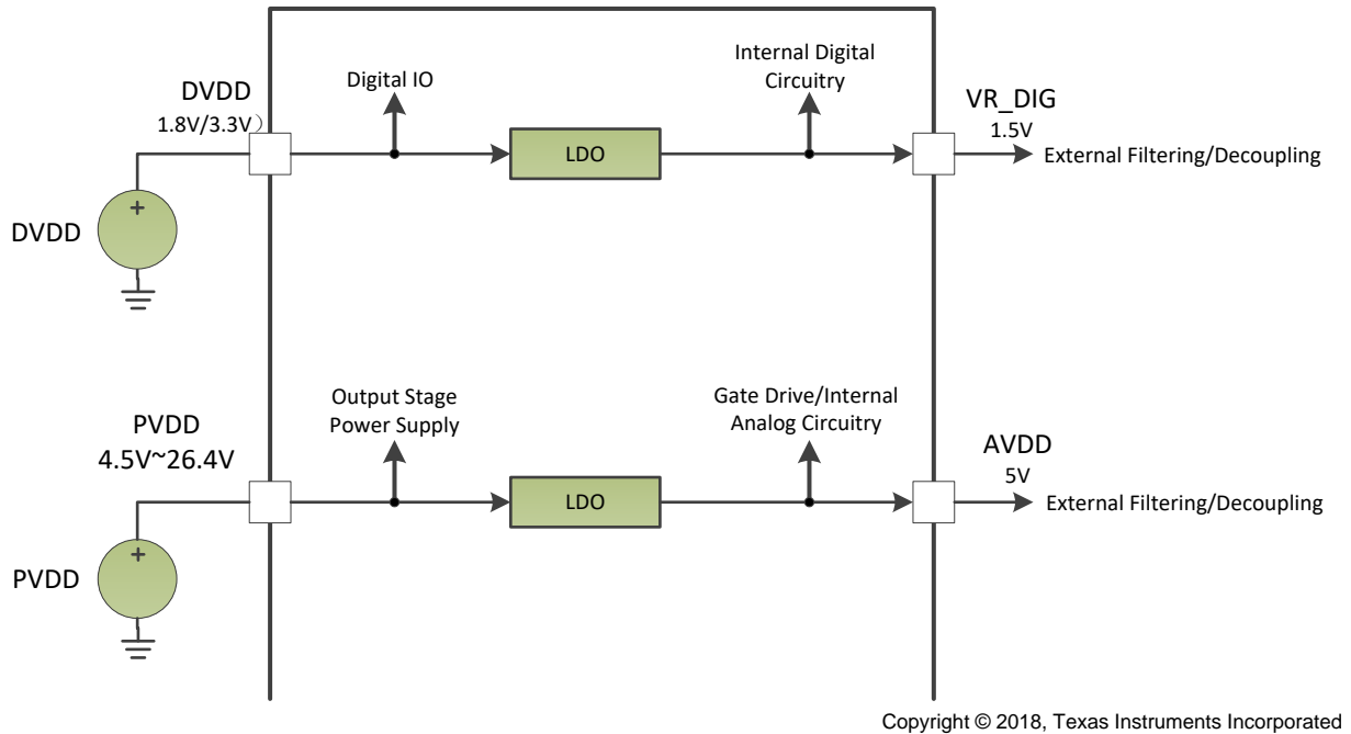
Figure 154. Power Supply Function Block Diagram
