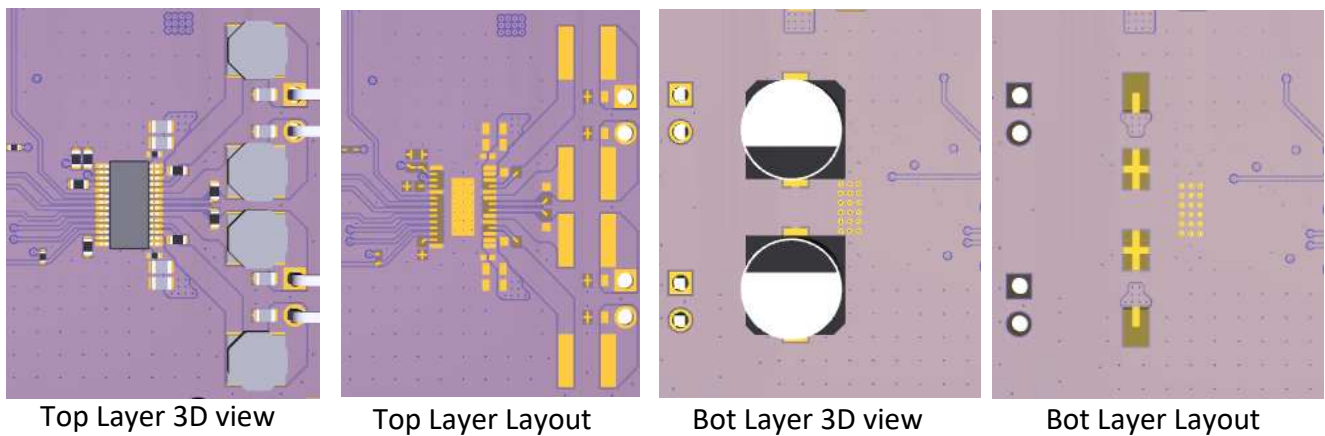
Figure 156. 2.0 (Stereo BTL with Inductor as Output Filter) Layout View
