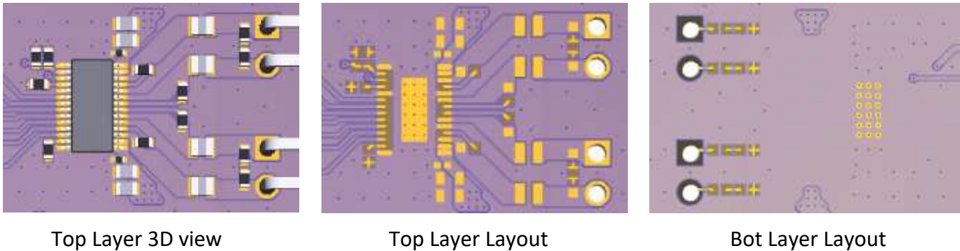
Figure 155. 2.0 (Stereo BTL with Ferrite Bead as Output Filter) Layout View
