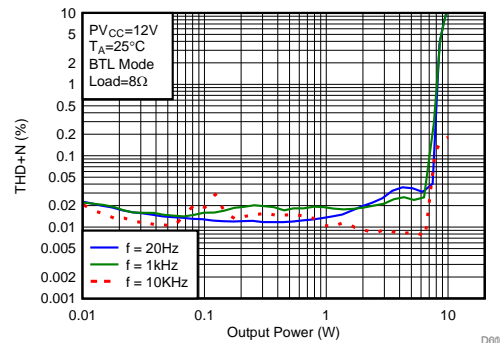
Figure 41. THD+N vs Output Power
