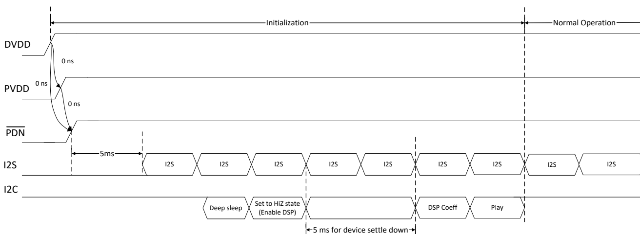
Figure 97. Start-up Sequence
