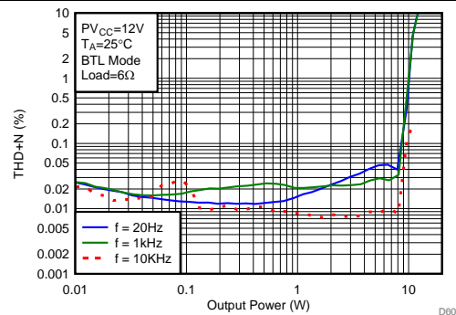
Figure 39. THD+N vs Output Power
