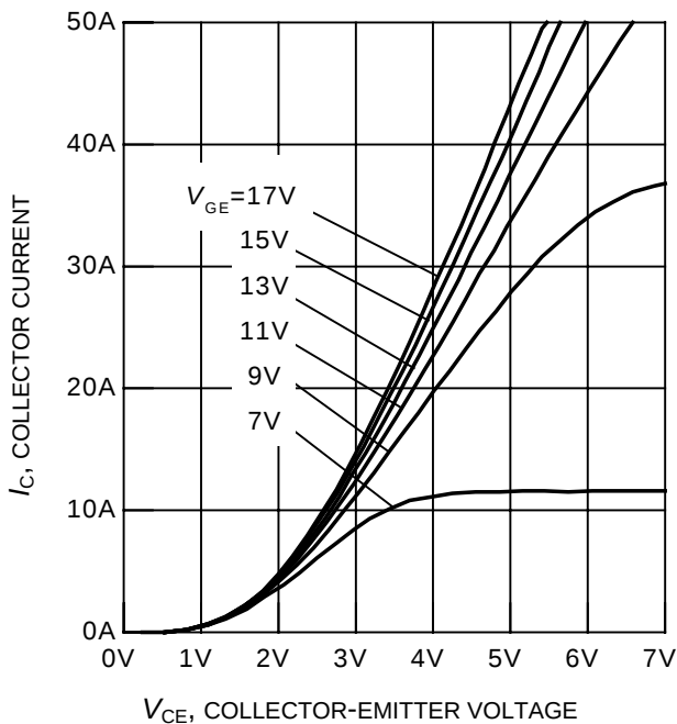
Figure 5. Typical output characteristics ( T_j = 25^\circ C )
