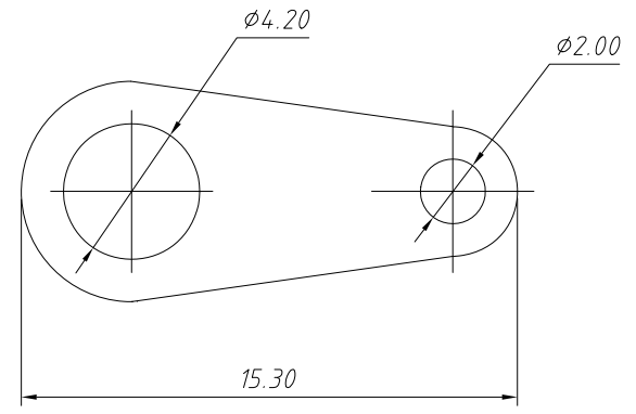
Solder Terminal
