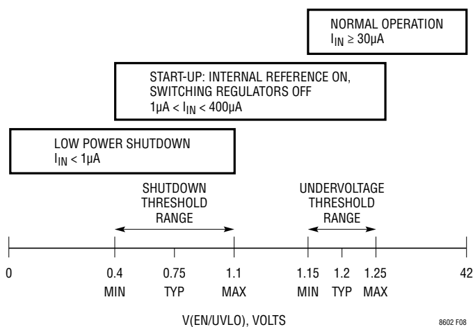
Figure 8. EN/UVLO Thresholds
