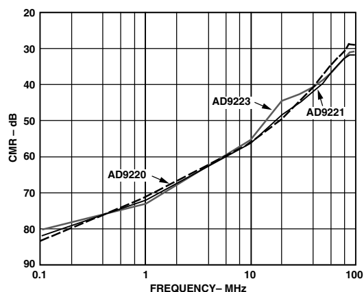
Figure 11. AD9221/AD9223/AD9220 Input CMR vs. Input Frequency
