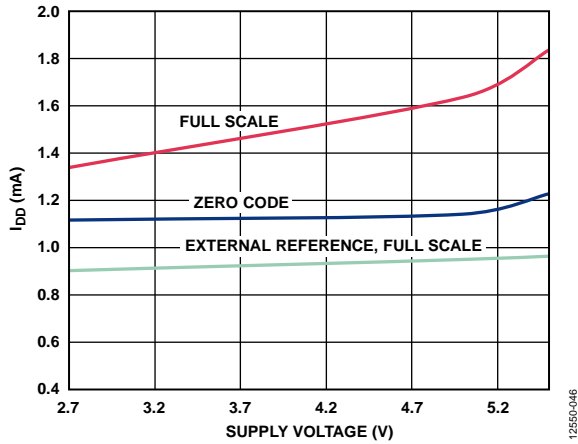
Figure 25. I_{DD} vs. Supply Voltage
