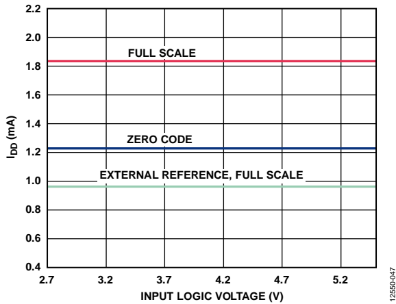
Figure 26. I_{DD} vs. Input Logic Voltage
