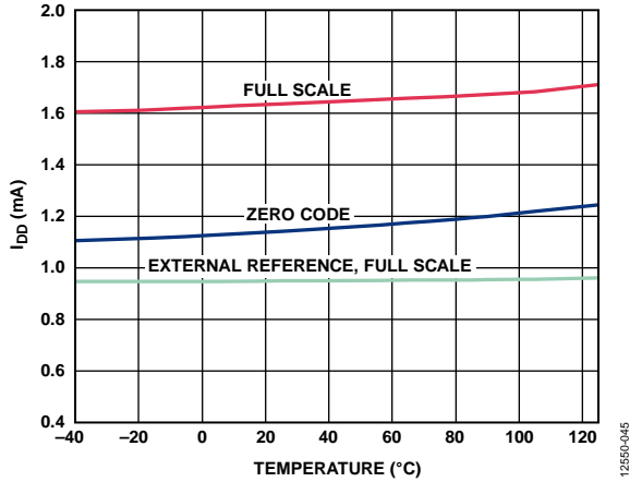
Figure 24. I_{DD} vs. Temperature
