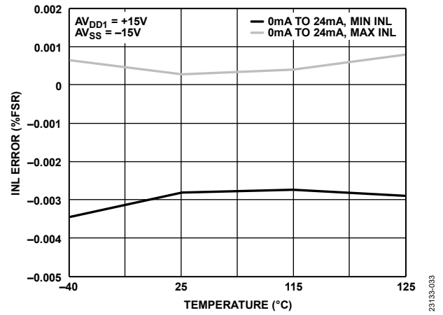
Figure 28. INL Error vs. Temperature, Internal RSET
