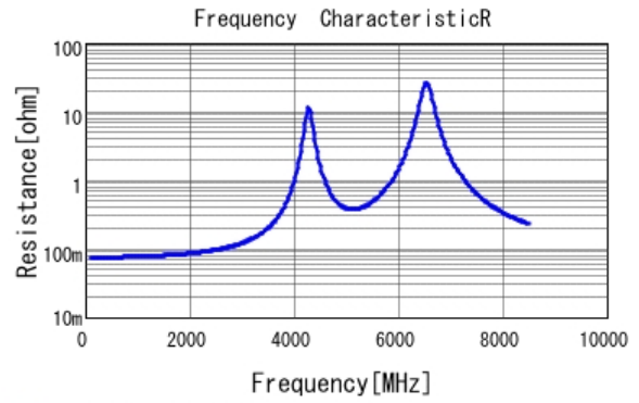
■ GCQ1555C1H220FB01 R DC0V, 25degC
