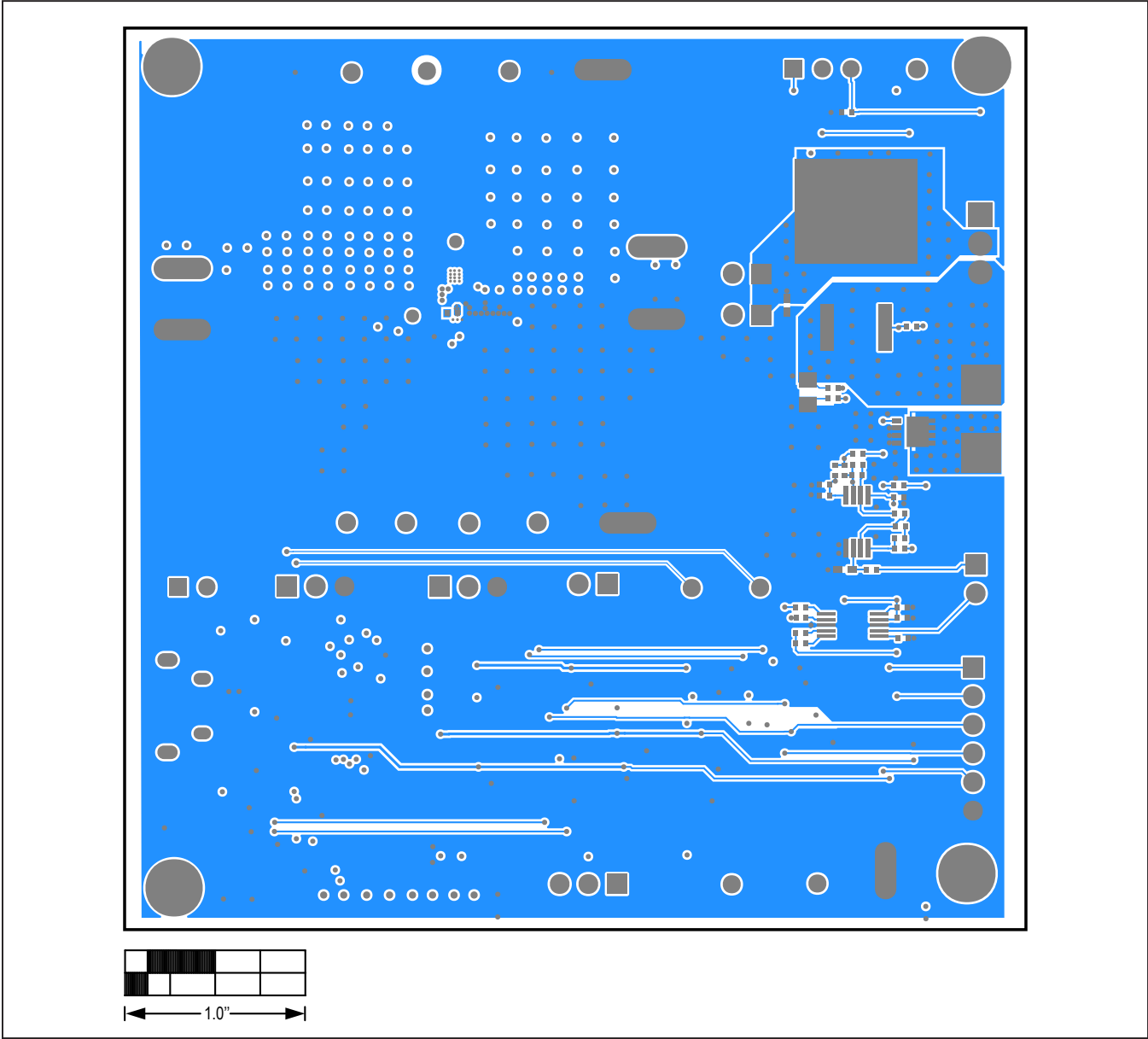
MAX77503 EV Kit PCB Layout—Bottom Layer
