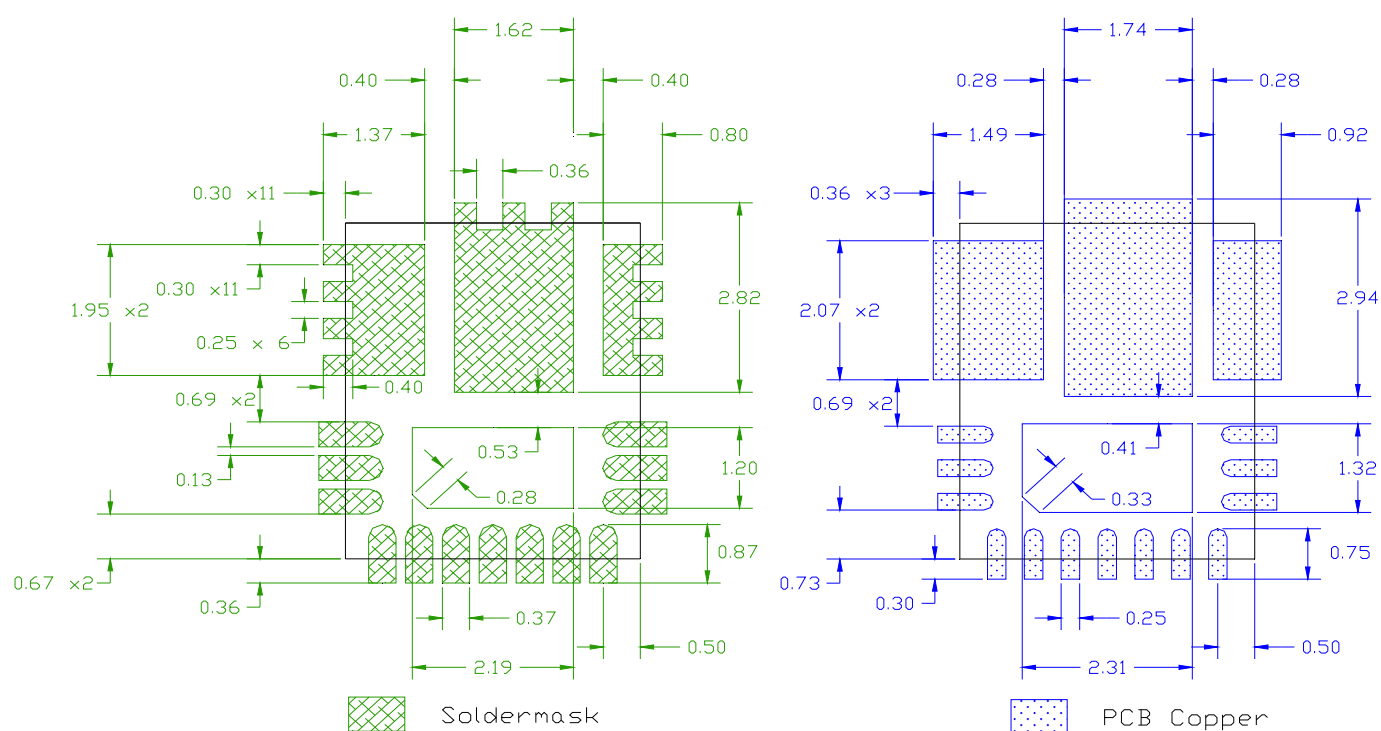
Figure 32: Solder Resist
