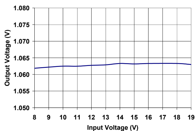
Figure 10: Line Regulation at I_{OUT} = 6A
