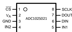
Figure 1. VSSOP Package See Package Number DGK0008A
