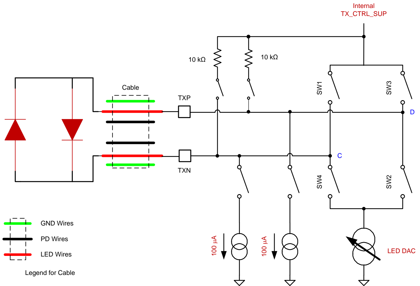
Figure 77. Transmitter Diagnostic
