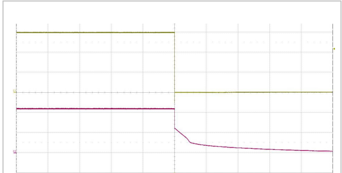
Shut-down enabled by disconnecting V_i at: T_{P1} = +25^\circ\text{C} , V_i = 110\text{ V} , I_o = 10\text{ A} resistive load. Top trace: output voltage (5 V/div.). Bottom trace: input voltage (50 V/div.). Time scale: (500 ms/div.).
