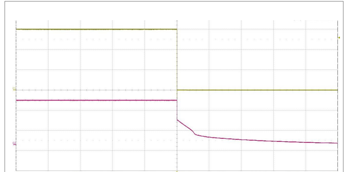
Start-up enabled by connecting V_i at: T_{P1} = +25^\circ\text{C} , V_i = 110\text{ V} , I_o = 6.67\text{ A} resistive load. Top trace: output voltage (5 V/div.). Bottom trace: input voltage (50 V/div.). Time scale: (500 ms/div.).
