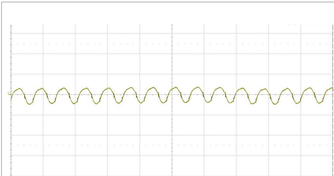
Output voltage ripple at: T_{P1} = +25^\circ\text{C} , V_i = 110\text{ V} , I_o = 10\text{ A} resistive load. Trace: output voltage (50 mV/div.). Time scale: (5 μs/div.).
