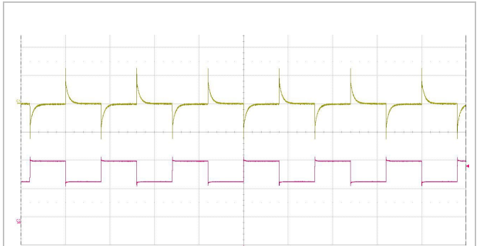
Output voltage response to load current step- change (1.56-2.34-1.56 A) at: T_{P1} = +25^{\circ}\text{C} , V_I = 110\text{ V} . Top trace: output voltage (500 mV/div.). Bottom trace: load current (1 A/div.). Time scale: (10 ms/div.).
