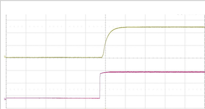
Start-up enabled by connecting V_i at: T_{P1} = +25^\circ\text{C} , V_i = 110\text{ V} , I_o = 12.5\text{ A} resistive load. Top trace: output voltage (5 V/div.). Bottom trace: input voltage (50 V/div.). Time scale: (50 ms/div.).
