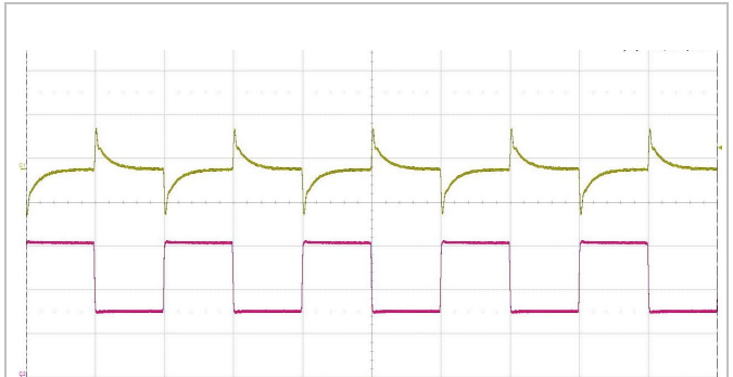
Output voltage response to load current step- change (3.125-4.68-3.125 A) at: T_{P1} = +25^\circ\text{C} , V_I = 110\text{ V} . Top trace: output voltage (500 mV/div.). Bottom trace: load current (1 A/div.). Time scale: (1ms/div.).
