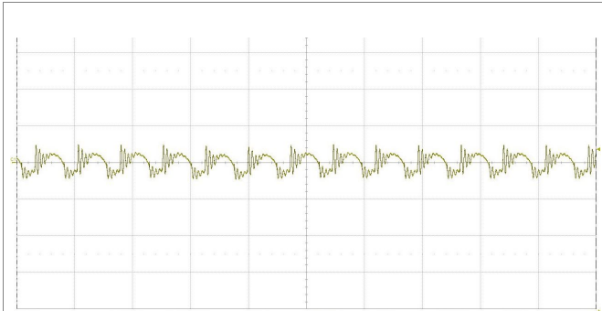
Output voltage ripple at: T_{P1} = +25^\circ\text{C} , V_I = 110\text{ V} , I_O = 20\text{ A} resistive load. Trace: output voltage (100 mV/div.). Time scale: (5 \mu\text{s} /div.).
