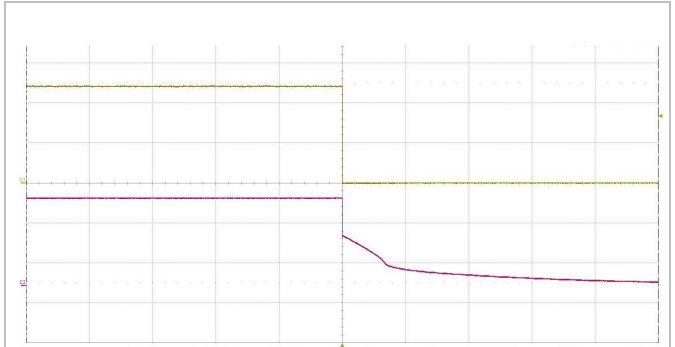
Shut-down enabled by disconnecting V_I at: T_{P1} = +25^\circ\text{C} , V_I = 110\text{ V} , I_O = 6.25\text{ A} resistive load. Top trace: output voltage (10 V/div.). Bottom trace: input voltage (50 V/div.). Time scale: (500 ms/div.).
