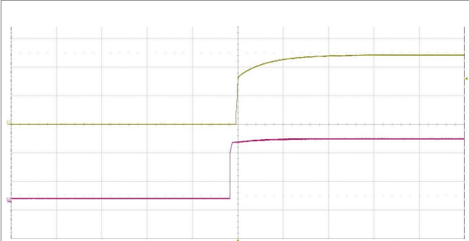
Start-up enabled by connecting V_i at: T_{P1} = +25^\circ\text{C} , V_i = 110\text{ V} , I_o = 4.16\text{ A} resistive load. Top trace: output voltage (10 V/div.). Bottom trace: input voltage (50 V/div.). Time scale: (20 ms/div.).
