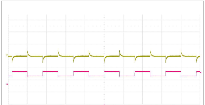
Output voltage response to load current step- change (1.04-1.56-1.04 A) at: T_{P1} = +25^{\circ}\text{C} , V_I = 110\text{ V} . Top trace: output voltage (2 V/div.). Bottom trace: load current (1 A/div.). Time scale: (10ms/div.).
