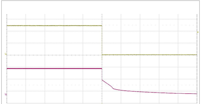
Shut-down enabled by disconnecting V_i at: T_{P1} = +25^\circ\text{C} , V_i = 110\text{ V} , I_o = 12.5\text{ A} resistive load. Top trace: output voltage (5 V/div.). Bottom trace: input voltage (50 V/div.). Time scale: (500 ms/div.).
