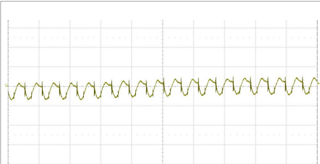
Output voltage ripple at: T_{P1} = +25^\circ\text{C} , V_i = 110\text{ V} , I_o = 4.16\text{ A} resistive load. Trace: output voltage (20 mV/div.). Time scale: (5 μs/div.).
