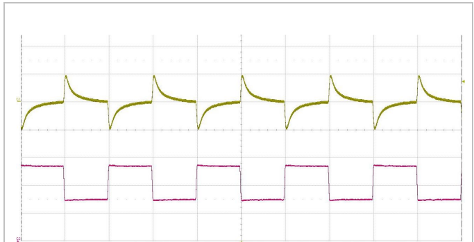
Output voltage response to load current step- Top trace: output voltage (500 mV/div.). change (5.0-7.5-5.0 A) at: Bottom trace: load current (2 A/div.). T_{P1} = +25^\circ\text{C} , V_i = 110\text{ V} . Time scale: (1ms/div.).
