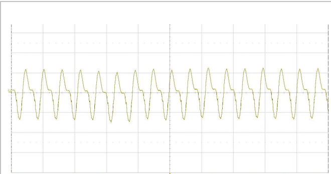
Output voltage ripple at: T_{P1} = +25^{\circ}\text{C} , V_I = 110\text{ V} , I_O = 2.08\text{ A} resistive load. Trace: output voltage (100 mV/div.). Time scale: (5 μs/div.).
