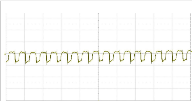
Output voltage ripple at: T_{P1} = +25^\circ\text{C} , V_I = 110\text{ V} , I_O = 6.25\text{ A} resistive load. Trace: output voltage (20 mV/div.). Time scale: (5 \mu\text{s} /div.).
