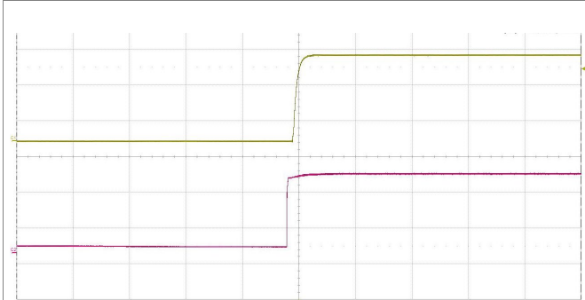
Start-up enabled by connecting V_i at: T_{P1} = +25^\circ\text{C} , V_i = 110\text{ V} , I_o = 8.3\text{ A} resistive load. Top trace: output voltage (5 V/div.). Bottom trace: input voltage (50 V/div.). Time scale: (50 ms/div.).
