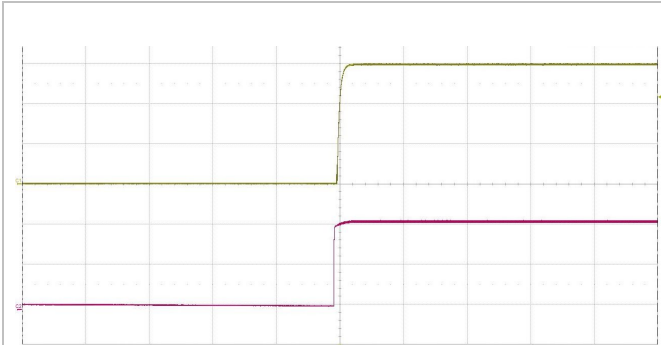
Start-up enabled by connecting V_i at: T_{P1} = +25^\circ\text{C} , V_i = 110\text{ V} , I_o = 10\text{ A} resistive load. Top trace: output voltage (5 V/div.). Bottom trace: input voltage (50 V/div.). Time scale: (100 ms/div.).
