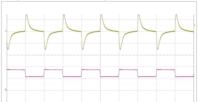
Output voltage response to load current step-change (6.25-9.375-6.25 A) at: T_{P1} = +25^\circ\text{C} , V_i = 110\text{ V} . Top trace: output voltage (500 mV/div.). Bottom trace: load current (5 A/div.). Time scale: (1ms/div.).
