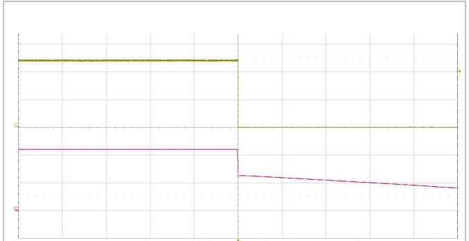
Shut-down enabled by disconnecting V_I at: T_{P1} = +25^{\circ}\text{C} , V_I = 110\text{ V} , I_O = 2.08\text{ A} resistive load. Top trace: output voltage (20 V/div.). Bottom trace: input voltage (50 V/div.). Time scale: (200 ms/div.).
