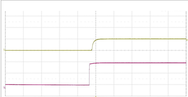
Start-up enabled by connecting V_I at: T_{P1} = +25^\circ\text{C} , V_I = 110\text{ V} , I_O = 20\text{ A} resistive load. Top trace: output voltage (5 V/div.). Bottom trace: input voltage (50 V/div.). Time scale: (50 ms/div.).
