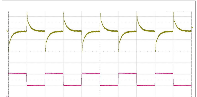
Output voltage response to load current step-change (2.08-3.12-2.08 A) at: T_{P1} = +25^\circ\text{C} , V_i = 110\text{ V} . Trace: output voltage (200 mV/div.). Bottom trace: load current (1 A/div.). Time scale: (1ms/div.).
