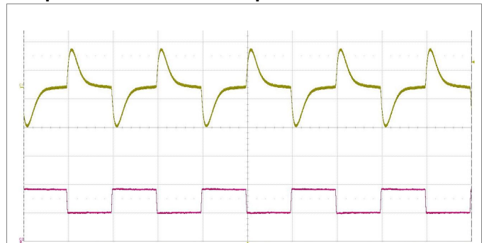
Output voltage response to load current step-change (3.335-5.003-3.335 A) at: T_{P1} = +25^\circ\text{C} , V_i = 110\text{ V} . Trace: output voltage (500 mV/div.). Bottom trace: load current (2 A/div.). Time scale: (1ms/div.).
