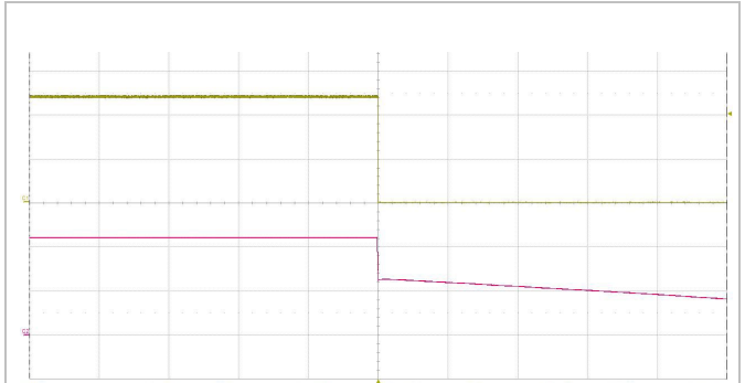
Shut-down enabled by disconnecting V_I at: T_{P1} = +25^{\circ}\text{C} , V_I = 110\text{ V} , I_O = 3.12\text{ A} resistive load. Top trace: output voltage (20 V/div.). Bottom trace: input voltage (50 V/div.). Time scale: (200 ms/div.).
