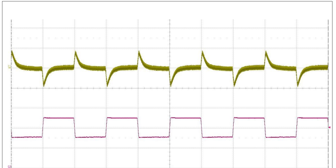
Output voltage response to load current step-change (10-15-10 A) at: T_{P1} = +25^\circ\text{C} , V_I = 110\text{ V} . Trace: output voltage (200 mV/div.). Bottom trace: load current (5 A/div.). Time scale: (1ms/div.).
