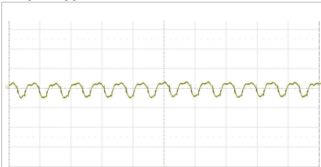
Output voltage ripple at: T_{P1} = +25^\circ\text{C} , V_i = 110\text{ V} , I_o = 8.3\text{ A} resistive load. Trace: output voltage (50 mV/div.). Time scale: (5 \mu\text{s} /div.).
