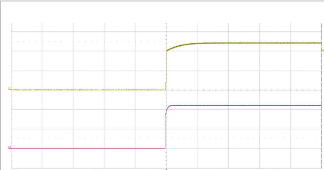
Start-up enabled by connecting V_I at: T_{P1} = +25^{\circ}\text{C} , V_I = 110\text{ V} , I_O = 2.08\text{ A} resistive load. Top trace: output voltage (20 V/div.). Bottom trace: input voltage (50 V/div.). Time scale: (200 ms/div.).
