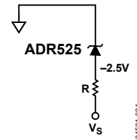
Figure 16. Negative Precision Reference Configuration
