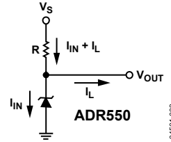
Figure 15. Shunt Reference
