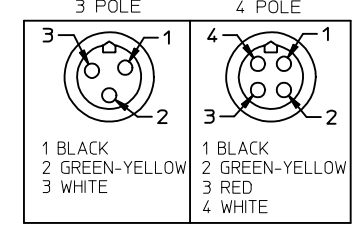
FACE VIEW-MALE INSERT
