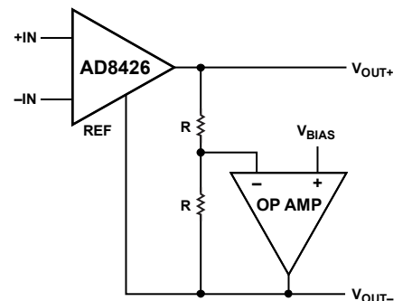
Figure 70. Differential Output Using an Op Amp
