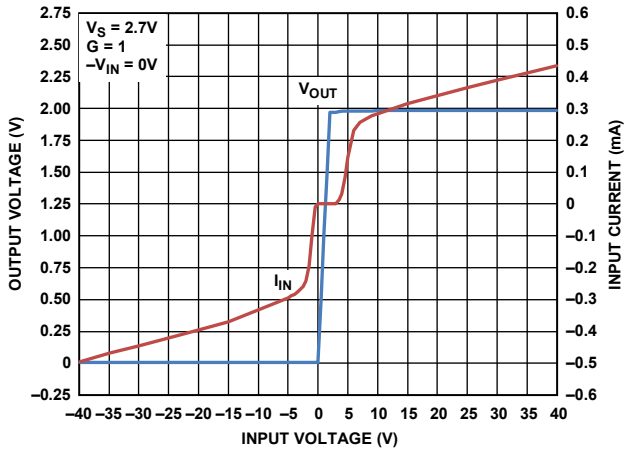
Figure 16. Input Overtolerance Performance, Single Supply, V_S = 2.7V , G = 1
