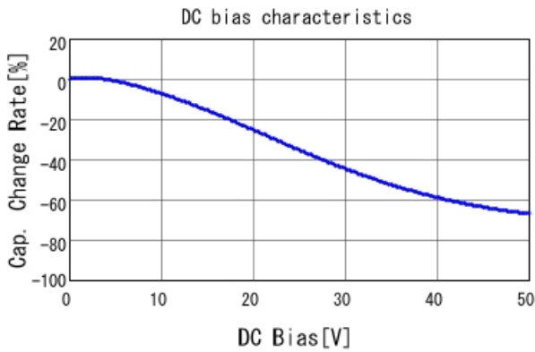
RDER71H225K2K1H03B C-DC bias capchange, 25.0degC,
