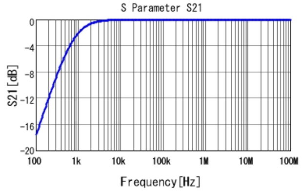
RDER71H225K2K1H03B S21 DC0V, 25degC
