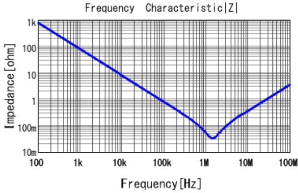
RDER71H225K2K1H03B |Z| DC0V, 25degC
