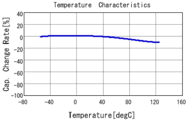
RDER71H225K2K1H03B C-Temp. capchange, DC0.0V, AC1.
