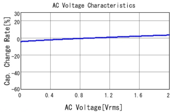
RDER71H225K2K1H03B C-AC Voltage capchange, DC0V, 2
