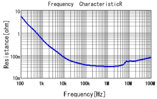
RDER71H225K2K1H03B R DC0V, 25degC
