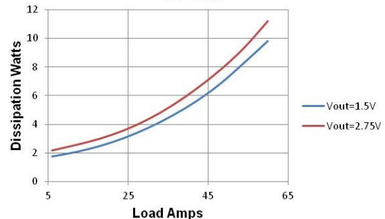
Figure 2. Power Dissipation at Vin = 8V Vin = 8.0V
