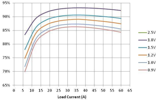
Figure 3. Efficiency vs Load at Vin = 12V
