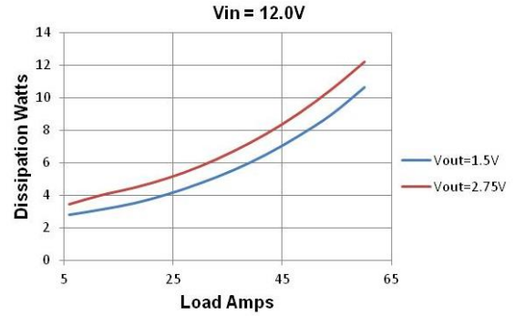
Figure 4. Power Dissipation at Vin = 12V
