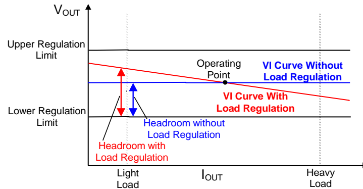
Figure 8. Concept of Optimal Voltage Positioning
