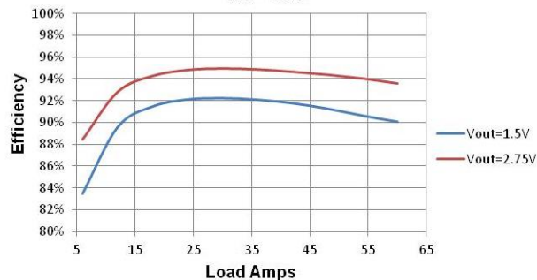
Figure 1. Efficiency at Vin = 8V Vin = 8.0V
