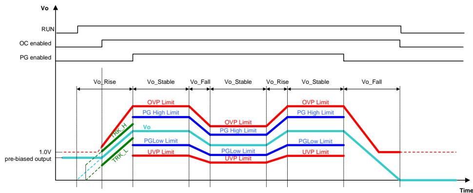
Figure 25. Protections Enable Conditions
