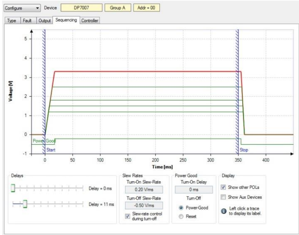
Figure 11. Sequencing/Tracking Window
