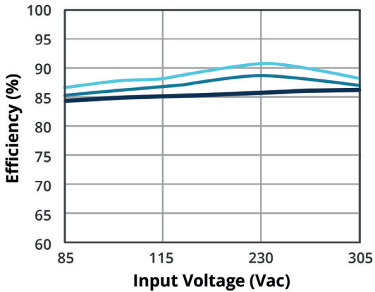
EFFICIENCY VS INPUT LOAD (full load)
