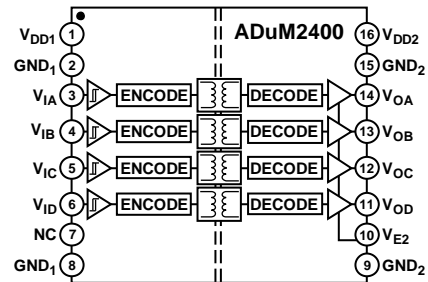
Figure 1. ADuM2400
