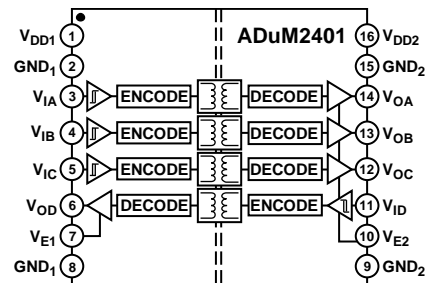
Figure 2. ADuM2401
