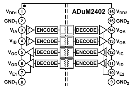
Figure 3. ADuM2402
