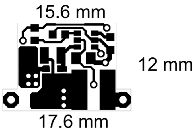
Figure 42. PCB Top Side MR 16 Application
