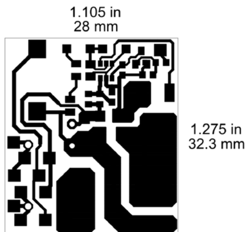
Figure 50. Single Layer PCB Design for this Application
