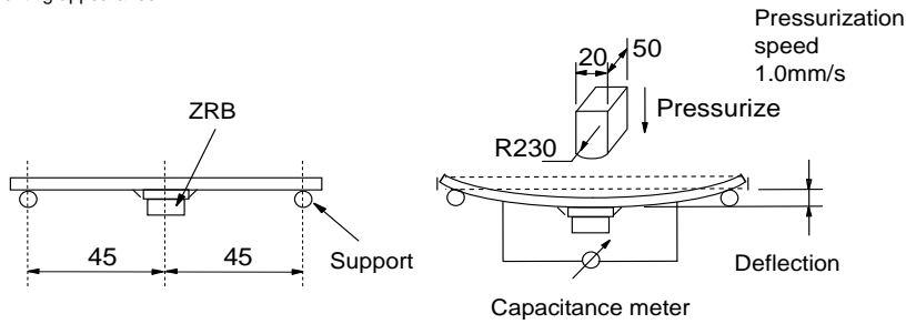
Fig.2 (in mm)
