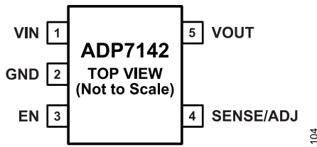
Figure 4. 5-Lead TSOT Pin Configuration
