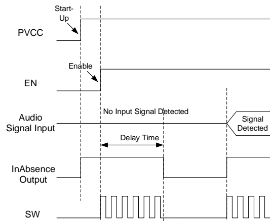
Figure 2: Enable On (No Signal Detected)
