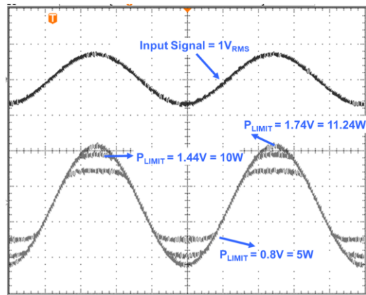
Figure 4: PLIMIT Circuit Operation
