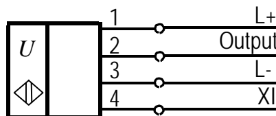
3RG6342-3AA00-PF:
