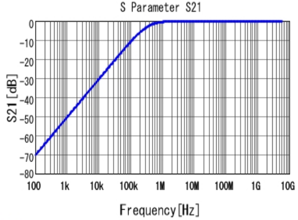
■ GCJ188R72A472KA01 S21 DC0V, 25degC
