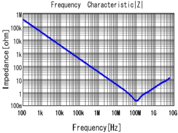
■ GCJ188R72A472KA01 |Z| DCOV, 25degC
