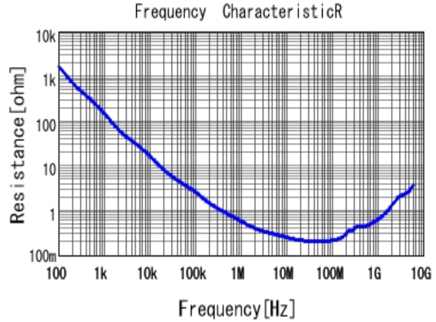
■ GCJ188R72A472KA01 R DCOV, 25degC
