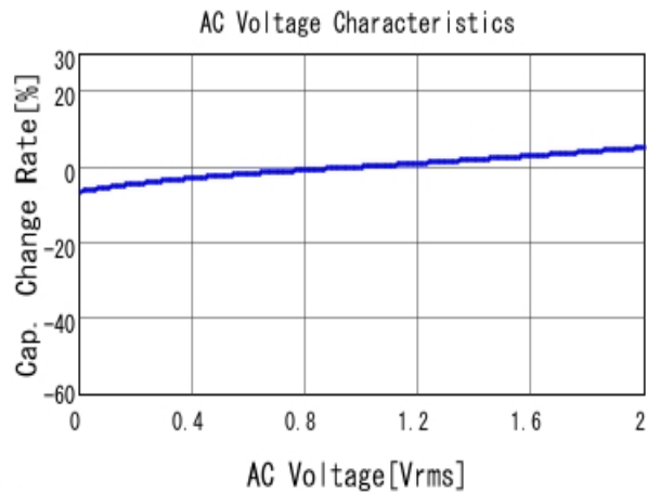
GCM21BR71C225KA64 C-AC Voltage capchange, DCOV, 25.0d
