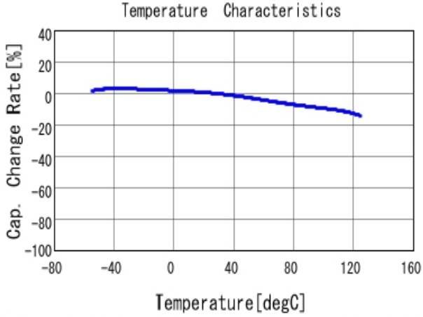
■ GCM21BR71C225KA64 C-Temp. capchange, DC0.0V, AC1.0V r m
