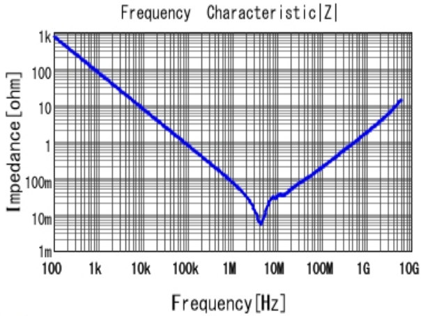
GCM21BR71C225KA64 |Z| DCOV, 25degC
