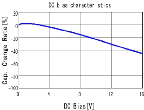
GCM21BR71C225KA64 C-DC bias capchange, 25.0degC, AC1.
