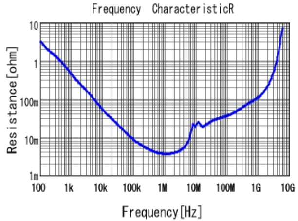
GCM21BR71C225KA64 R DCOV, 25degC
