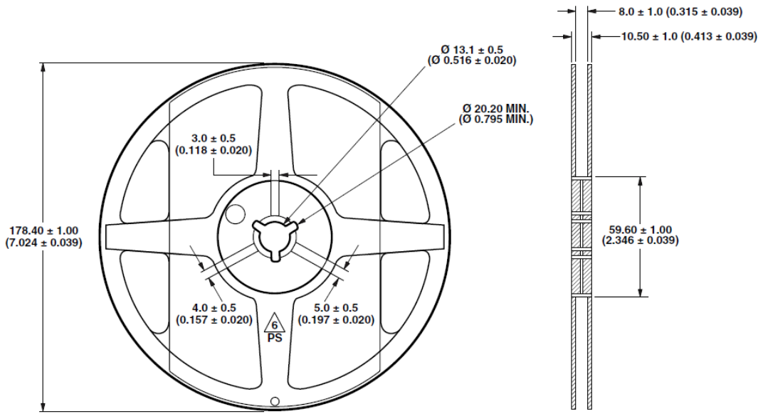
Figure 13: Reel Dimensions
