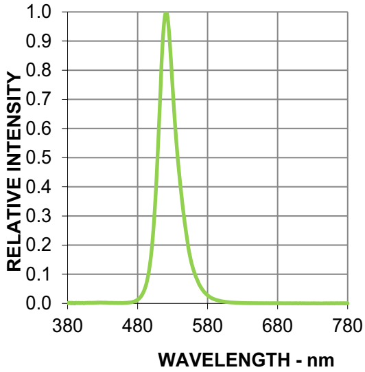
Figure 2: Spectrum
