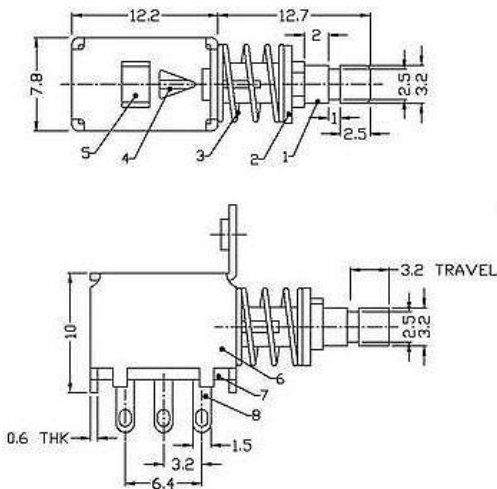
Outline Drawing
