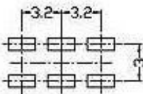
Mounting
