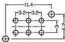
Mounting
