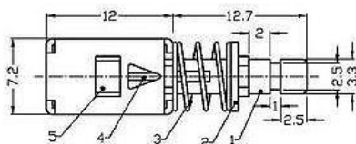
Outline Drawing
