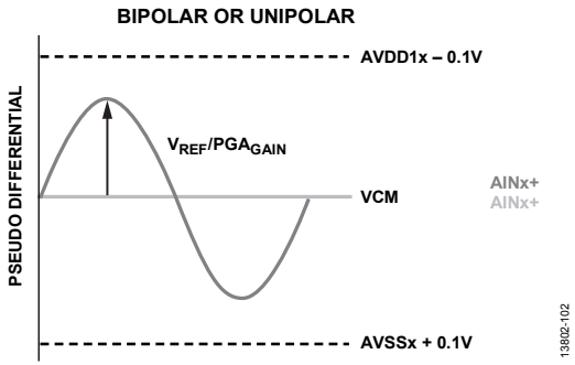
Figure 102. Σ-Δ ADC Input Signal Configuration, Pseudo Differential
