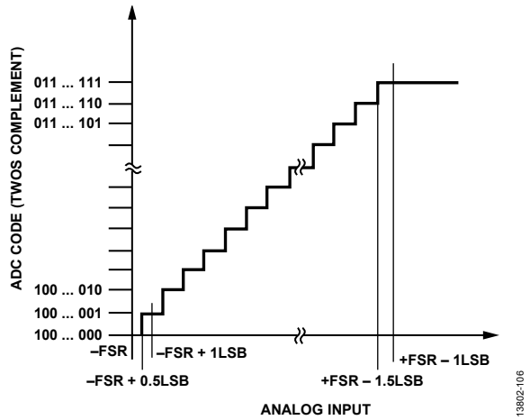
Figure 106. Transfer Function
