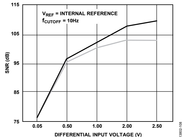
Figure 108. SNR Adding External LPF with V_{\text{REF}} = \text{Internal Reference} and f_{\text{CUTOFF}} = 10 Hz
