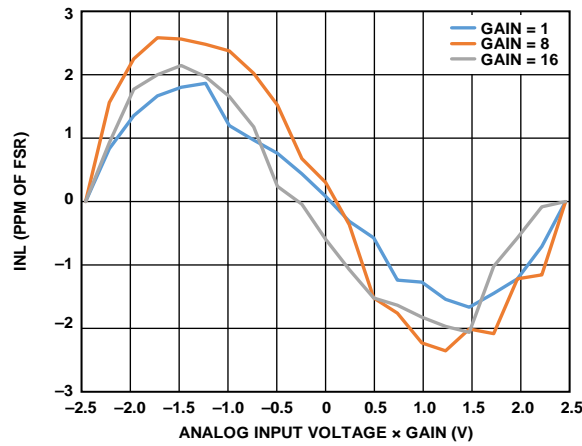
Figure 26. INL vs. Differential Input Signal (Analog Input \times Gain), ODR = 50 SPS, External 2.5 V Reference
