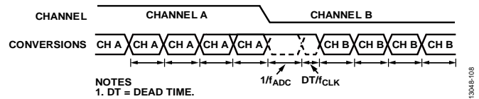
Figure 101. Fast Settling, Sinc 4 + Sinc 1 Filter
