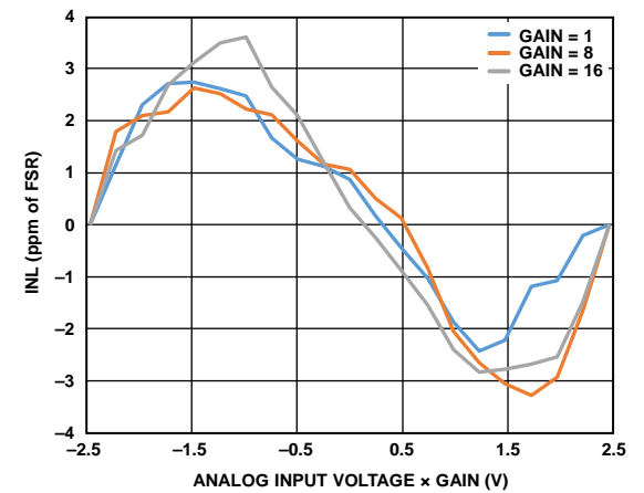
Figure 27. INL vs. Differential Input Signal (Analog Input \times Gain), ODR = 50 SPS, Internal Reference
