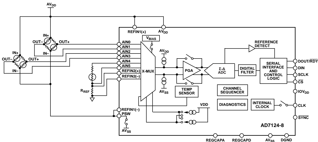
Figure 131. Flowmeter Application
