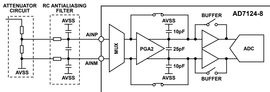
Figure 76. Input Schematic
