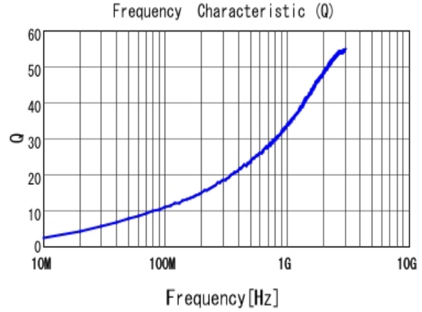
■ LQP03TN2N2C02 Q
