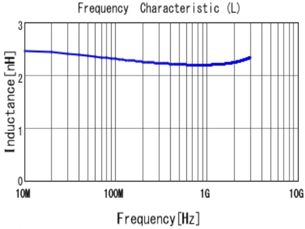
■ LQP03TN2N2C02 L
