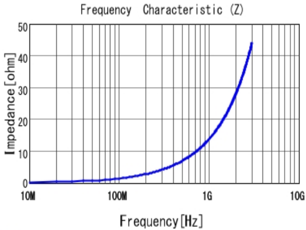
■ LQP03TN2N2C02 |Z|
