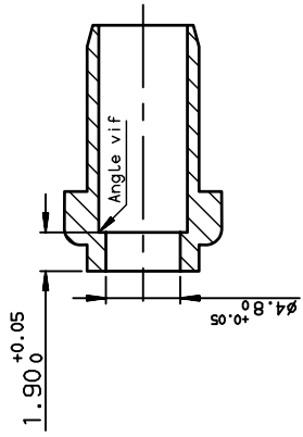
Detail section A-A
