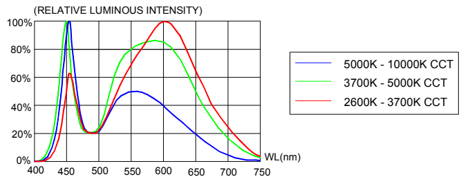
FIG.4 RELATIVE LUMINOUS INTENSITY VS. WAVELENGTH.
