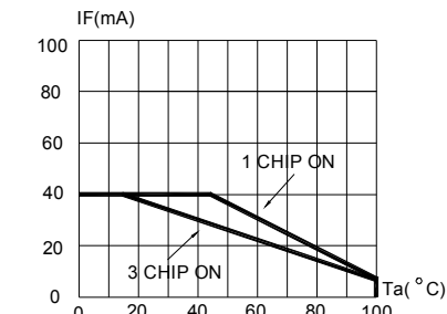
FIG.6 BLUE & GREEN BLUE & GREEN MAXIMUM FORWARD DC CURRENT VS AMBIENT TEMPERATURE
