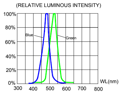
FIG.4 BLUE&GREEN RELATIVE LUMINOUS INTENSITY VS. WAVELENGTH.
