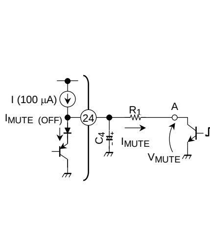
Figure 4 Muting Function
