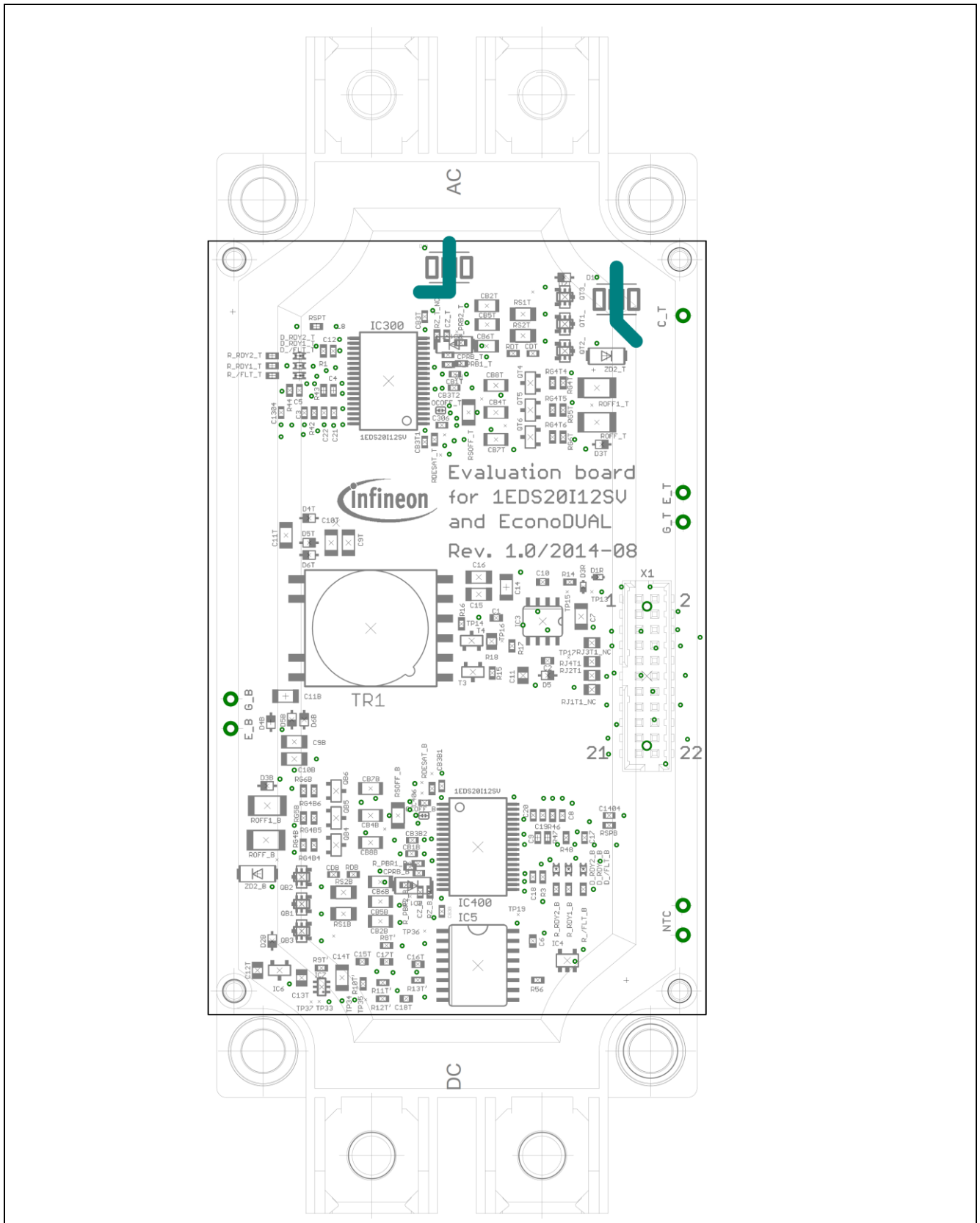
Figure 19 Assembly print
