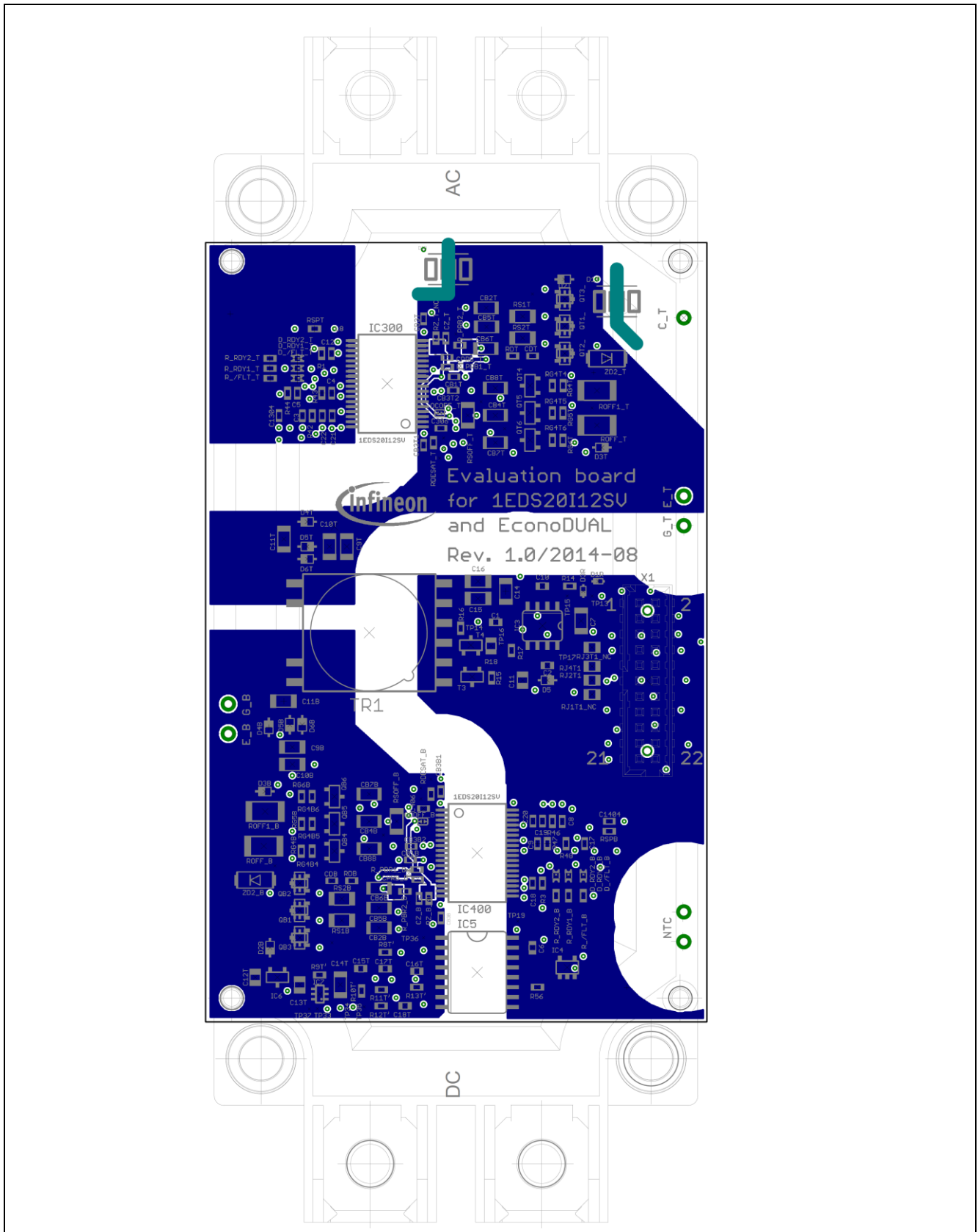
Figure 18 Bottom layer
