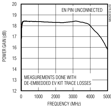
MAX2616 GAIN vs. FREQUENCY
