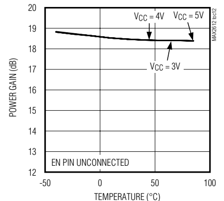
MAX2613 GAIN vs. TEMPERATURE
