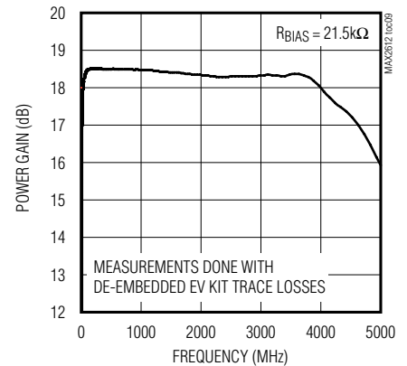
MAX2615 GAIN vs. FREQUENCY
